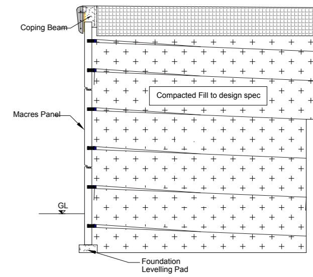
MacRes Reinforced Soil Wall
