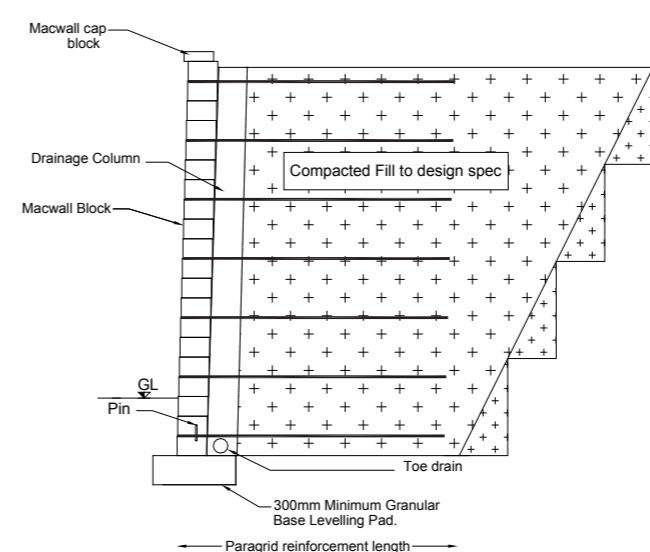
MacWall Reinforced Soil Wall
