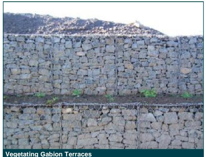
Vegetating Gabion Terraces
